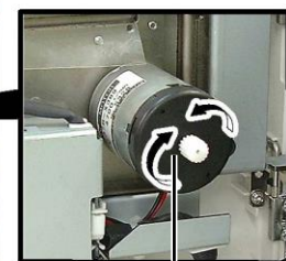
Cutter Motor Shaft
